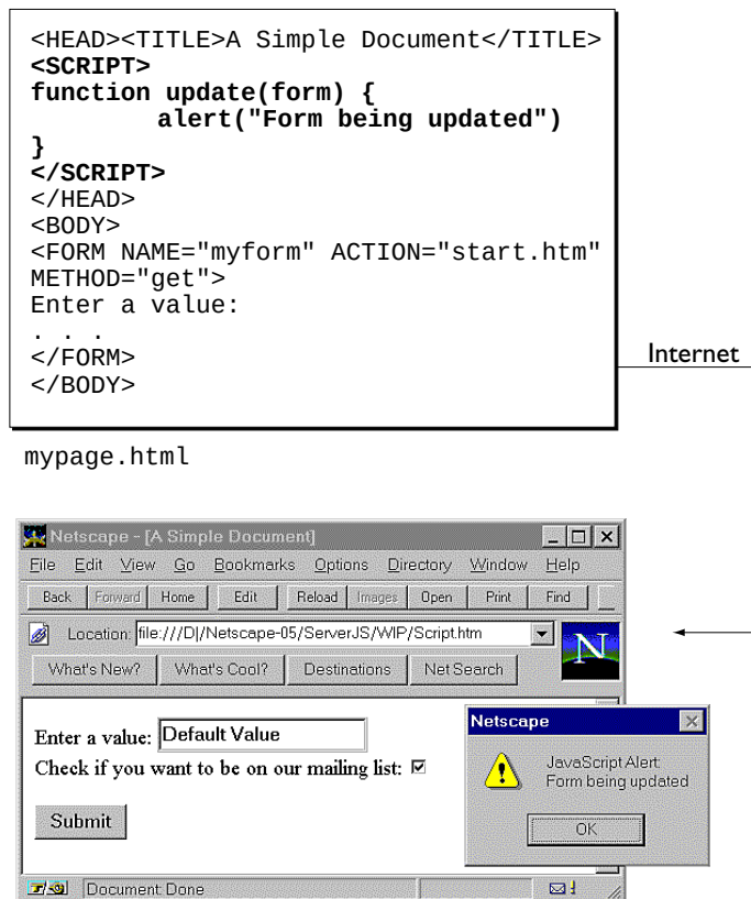
Figure 1.2 Client-side JavaScript
